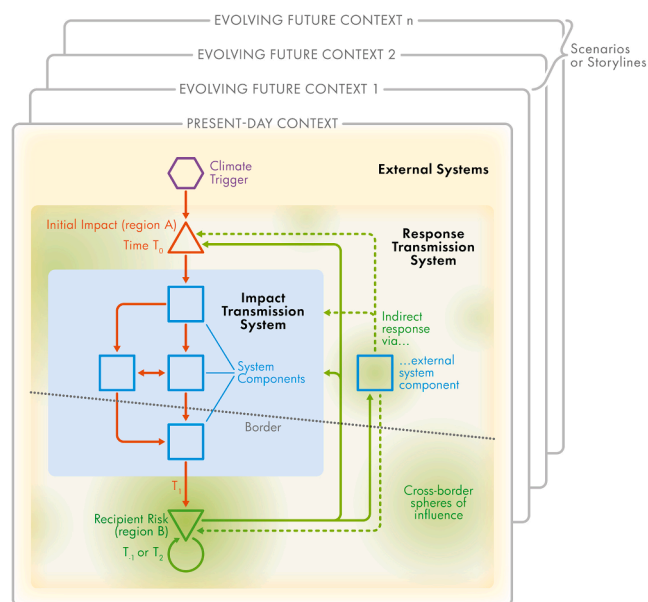
Fig. 2. Conceptual framework for the transmission of cross-border impacts and responses. An initial impact in one region due to a climate trigger is propagated (red arrows) via an impact transmission system (blue area) comprising impacts on interconnected system components of varied complexity, resulting in a recipient risk in a second region (location of the border is notional). Adaptive responses for ameliorating that risk (green arrows) can be targeted within a response transmission system (green area) directly at the recipient risk itself, at the impact transmission system and at the site of initial impact (solid arrows), and indirectly via system components external to the impact transmission system (dashed arrows). Responses can occur prior ( T_1 ) or subsequent ( T_2 ) to the times of the initial impact ( T_0 ) and recipient risk ( T_1 ), to indicate anticipatory or reactive adaptation. The ability to respond can vary in terms of the sphere of influence exerted by the regional actor managing the recipient cross-border risk (strength of background green shading tone). Note that a response with longer-term effectiveness, operating directly on the climate trigger and not shown here, would be greenhouse gas mitigation. Transmission systems are shown in relation to external systems that may include non-climate drivers of key importance in understanding both the propagating impacts and necessary responses. The present-day context in which the systems operate is coloured yellow and evolves into an uncertain future, depicted as stacked scenarios or storylines.
